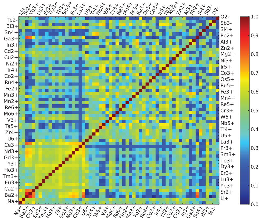
FIG. 2. (Color online) Rescaled ionic substitutional similarity function. The probability of ion a substituting for ion b within the same prototype, rescaled to better differentiate substitution probabilities.
