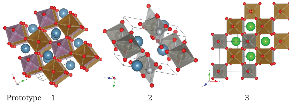
FIG. 3. (Color online) Three crystal structure prototypes suggested by the composition similarity method for the crystal structure of \text{Ca}_2\text{FeWO}_6 . The first and third prototypes are both double perovskites, with the octahedron in the first prototype being slightly distorted. The second prototype represents an experimentally determined polymorph of \text{Ca}_2\text{NiWO}_6 .
