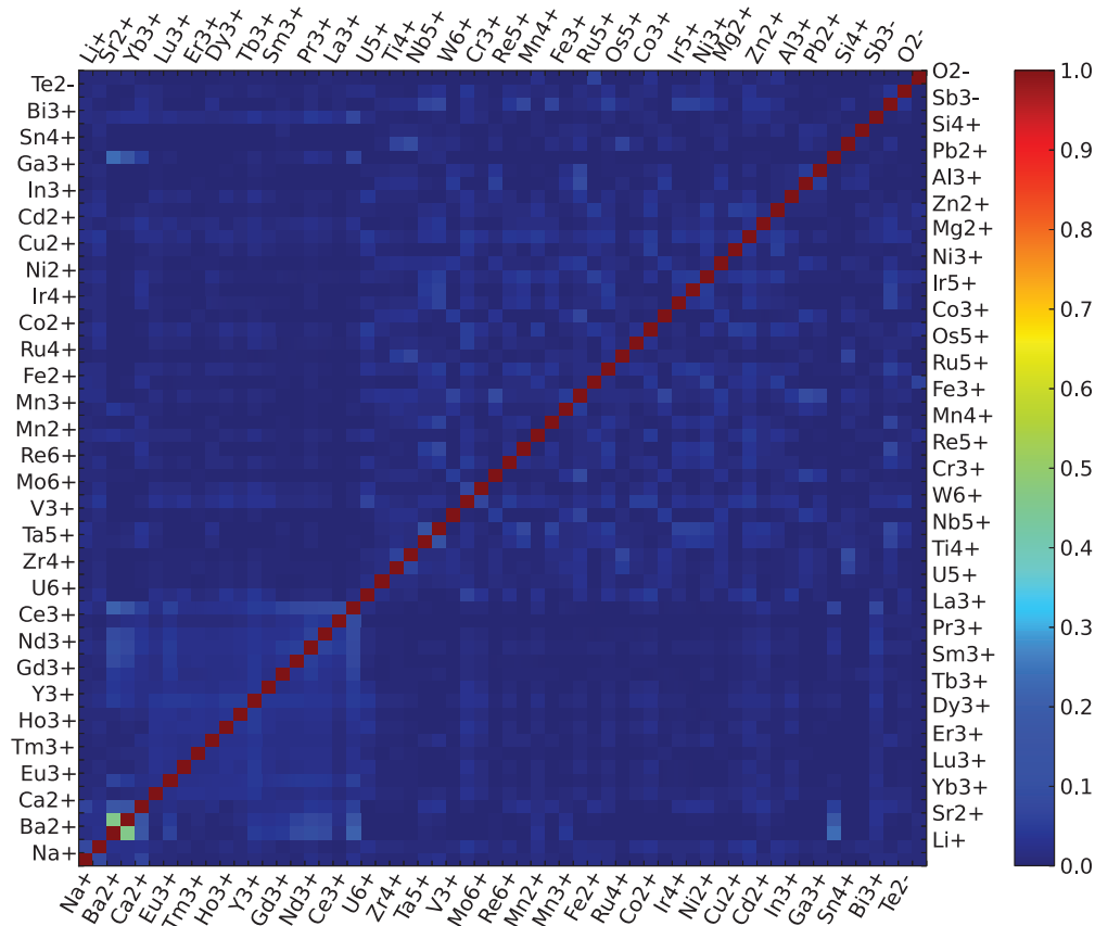
FIG. 1. (Color online) Unscaled ionic substitutional similarity. The probability of ion a substituting for ion b within the same structure prototype as given by the maximum likelihood model applied to the oxides in the ICSD.
