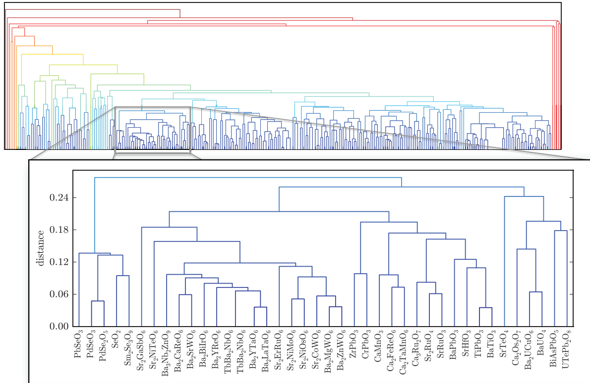
FIG. 7. (Color online) Clustering of a sample set of 300 oxides from the ICSD by composition similarity.
