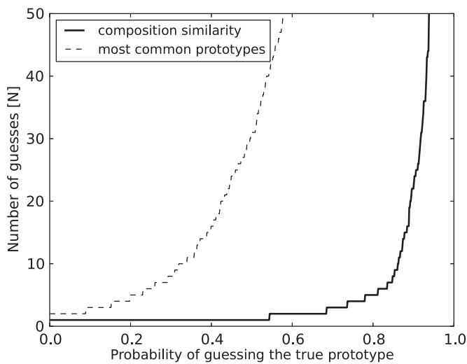
FIG. 5. Prototyping by composition similarity as applied to the oxides in the ICSD. The black line shows the number of guesses necessary to select the correct prototype by composition similarity. The dotted line shows the number of guesses necessary if those guesses were ordered by the frequency with which that prototype appears.
