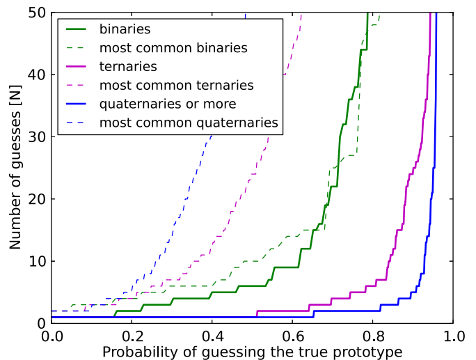
FIG. 6. (Color online) Prototyping by composition similarity broken down by the number of components in a compound. The bold lines show the number of guesses necessary to select the correct prototype by composition similarity. The dotted lines show the number of guesses necessary if those guesses were ordered by the frequency with which that prototype appears. The performance of composition similarity increases dramatically with the number of components in a compound.
