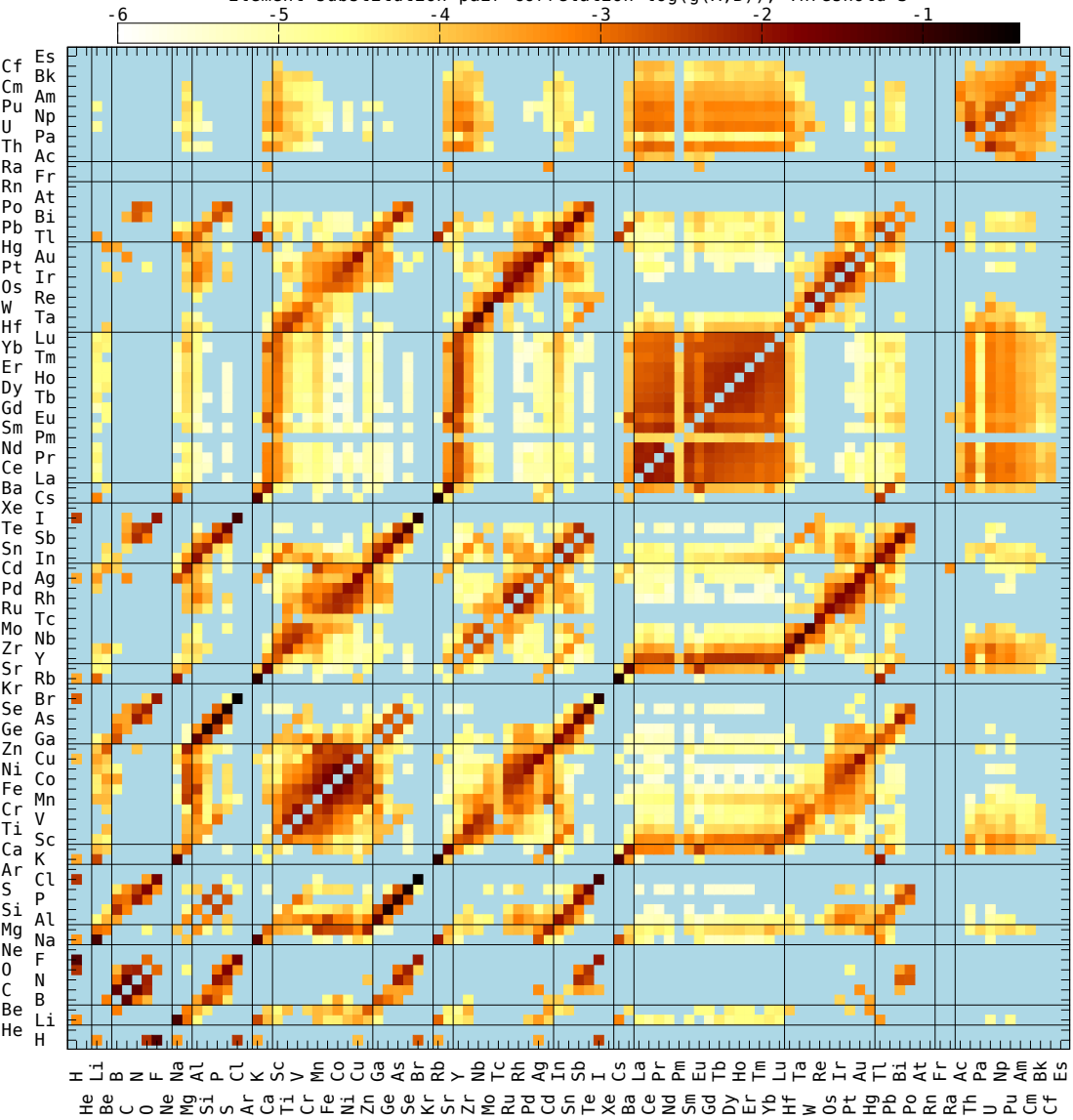
Element substitution pair correlation \log(g(A,B)) , Threshold 3
