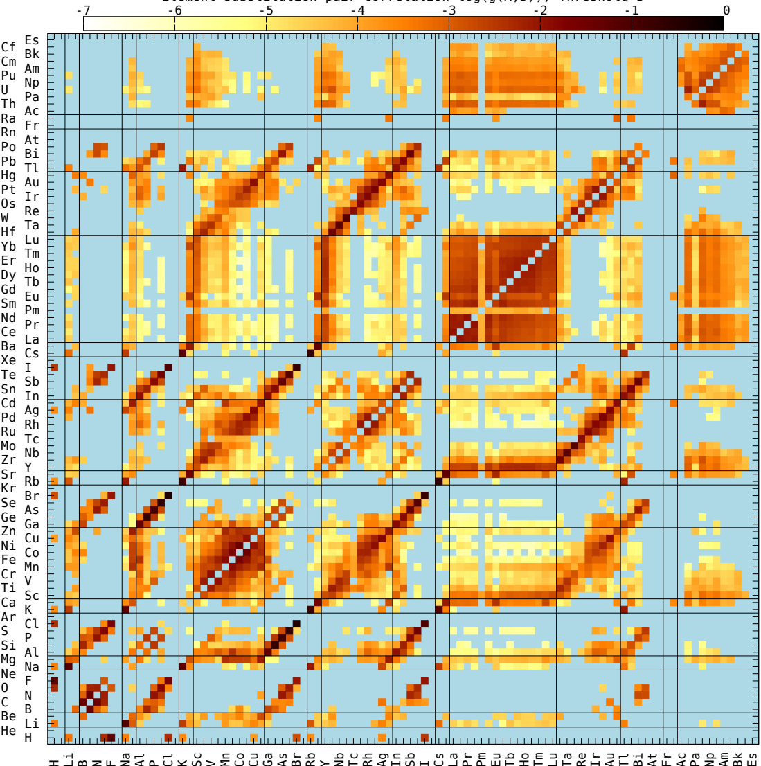
Element substitution pair correlation \log(g(A,B)) , Threshold 3
